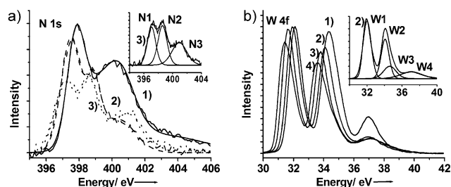
Figure 3. XPS a) N 1s spectra of 1) CN, 2) WCN and 3) Fe-WCN materials prepared at 800 °C; the inset shows the deconvoluted XPS N 1s spectra of Fe-WCN-800 (3). b) W 4f spectra of Fe-WCN catalysts prepared at various temperatures. 1) Fe-WCN-700, 2) Fe-WCN-800, 3) Fe-WCN-900, and 4) Fe-WCN-1000. The inset shows the deconvoluted XPS W 4f spectra of Fe-WCN-800 (2). W1 and W2 are N-bound W atoms, W3 and W4 are O-bound W atoms.
