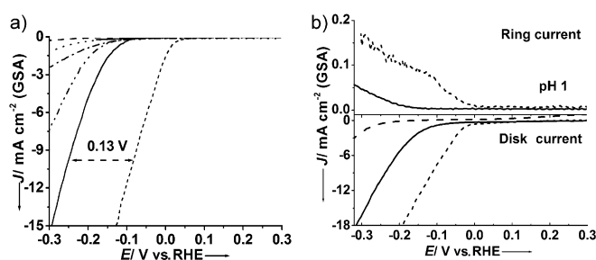
Figure 2. a) HER polarization curves of glassy carbon (---), CN-800 (.....), FeCN (-.-.-), WCN-800 (—), Fe-WCN-800 (—), and commercial Pt/C (----) catalyst in a pH 1 medium. b) H 2 gas evolved on the disk electrodes of a RRDE system; Fe-WCN (—), Pt/C (20 wt %; ----), c-Fe-WCN (-.-.-). Scan rate = 5 mV s -1 , rotational speed = 1000 r.p.m., catalyst loading = 0.4 mg cm -2 . c-Fe-WCN = conventional Fe-WCN, GSA = geometric surface area (0.2 cm 2 ).
